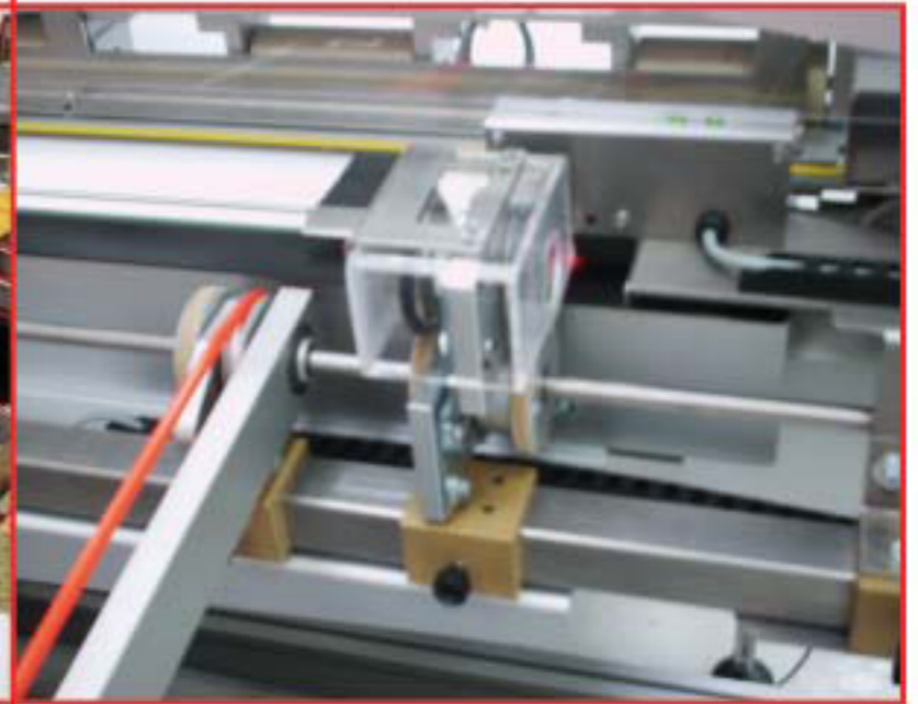
The exit sorting tools (optional) position the jobs on the collecting table.
